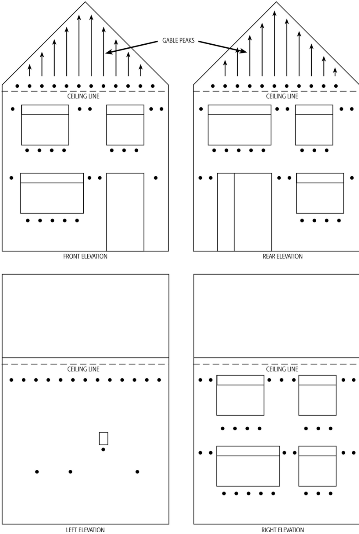
Figure 1: Typical Aerobead / Aerobead Plus Hole Drilling Pattern in a Detached Dwelling
